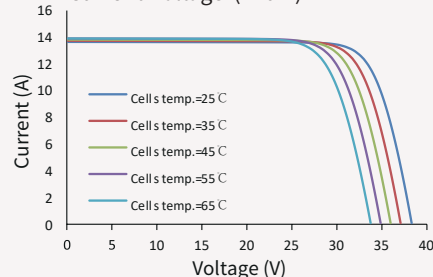
Current-Voltage (420W)
