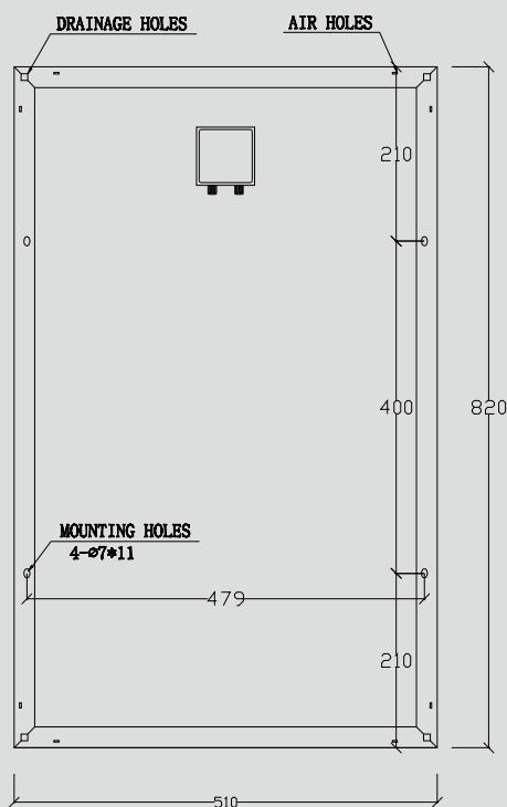
Engineering Drawings (Back Side)
