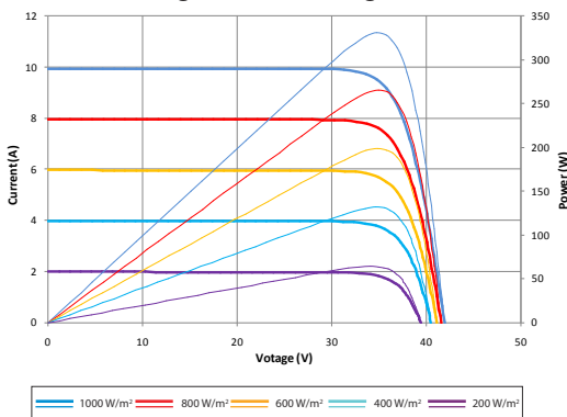
Current-Voltage & Power-Voltage Curve (330S)
