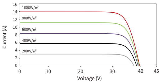
Current-Voltage Curves (54HL4R-V 450W)
