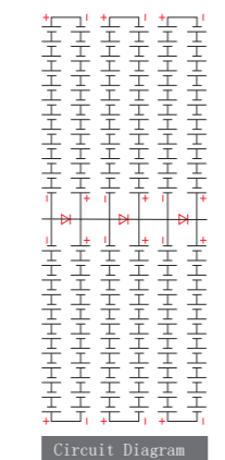
Circuit Diagram
