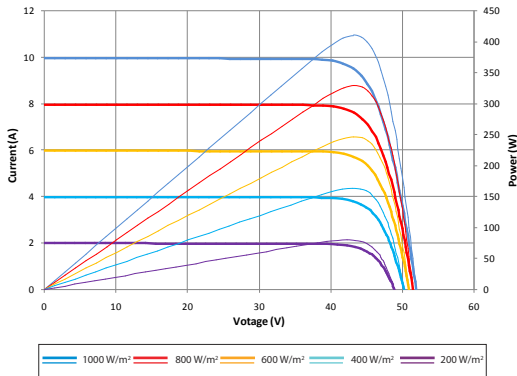
Current-Voltage & Power-Voltage Curve (410S)
