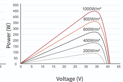
P-V Curves (455W)
