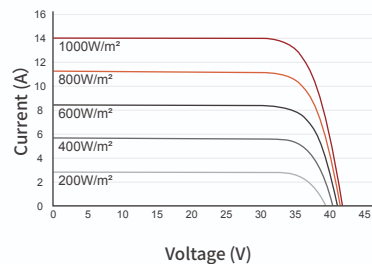
I-V Curves (455W)
