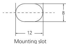
Mounting slot
